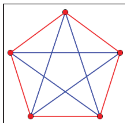
Figure 1. Ramsey graph r(3,3) with five vertices. Figure courtesy of Jacques Verstraete.
