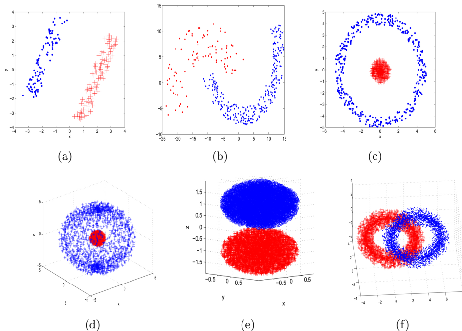
Figure 5 Accurate clustering results for data sets of many shapes and sizes using spectral clustering: (a) Gaussian strips, (b) Interlocked half rings, (c) Concentric rings, (d) Concentric spheres, (e) Tangent spheres, and (f) Interlocked rings.
